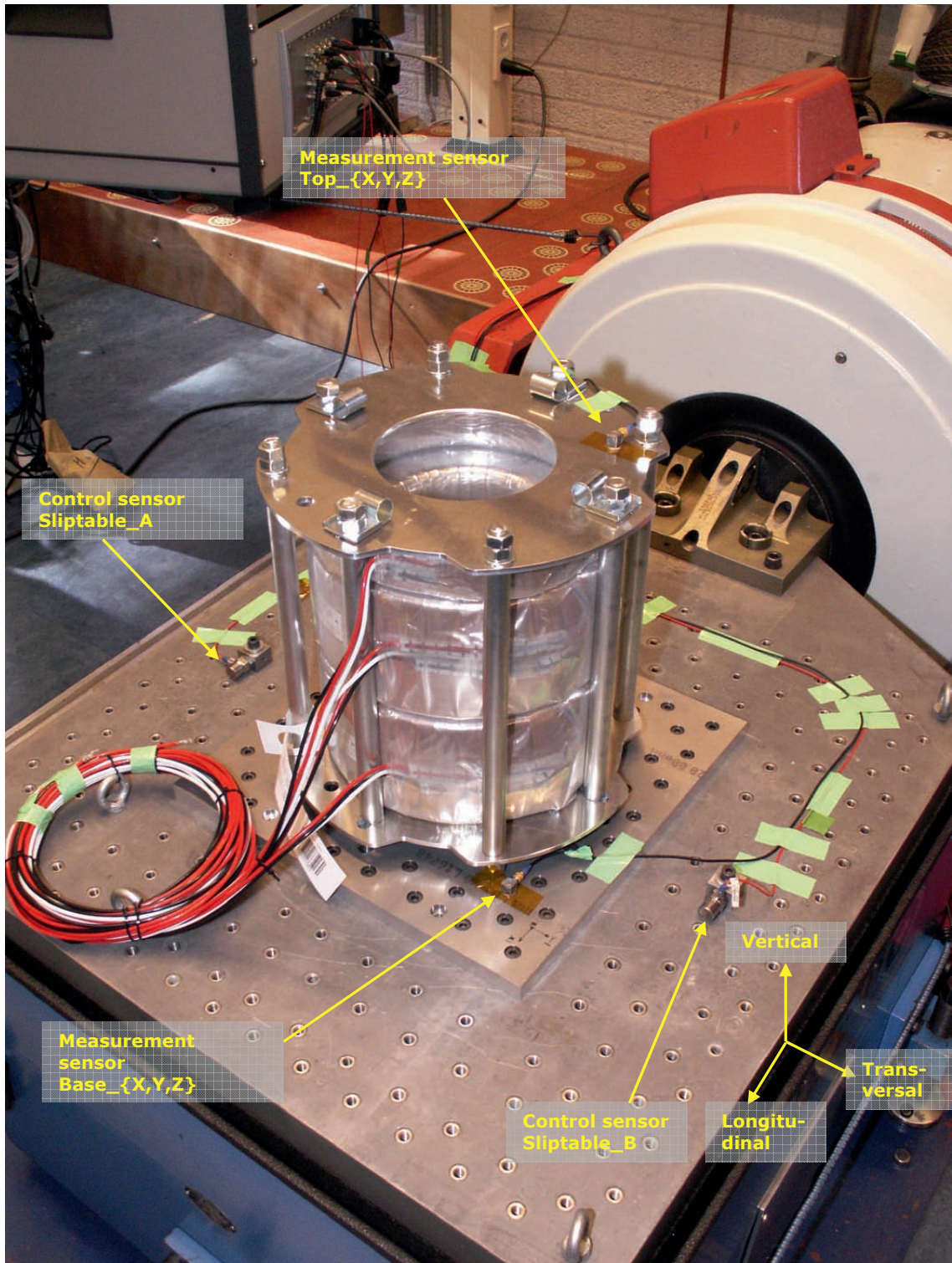
Fig. B.1 Transformer on Slip table in X-direction (Longitudinal)
